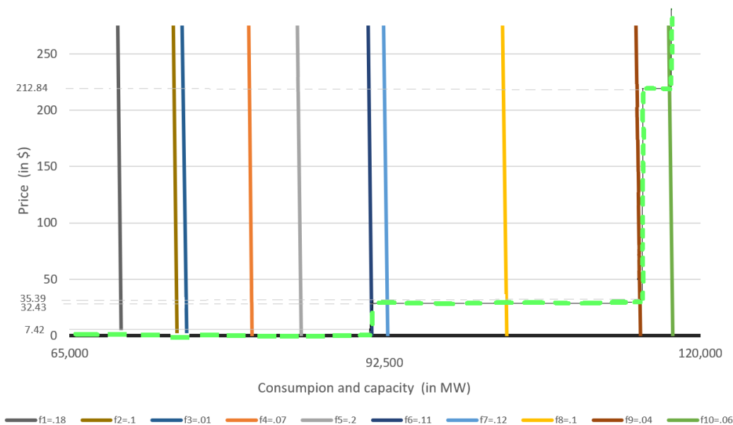
Figure 1: The status quo long-run equilibrium that would arise in an energy-only market given the ten demand states and three types of economic generators that result based on the cost and demand profiles in PJM. Each color corresponds to a different demand state with the frequency of the occurrence given below the graph. The green dashed line is the equilibrium supply curve.
