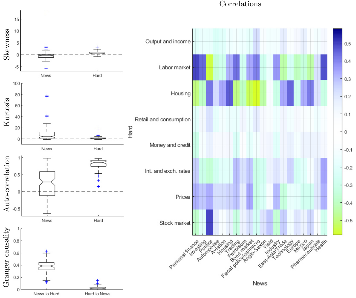
Figure 2.2. Descriptive statistics. The box plots report skewness, kurtosis and the first-order auto-correlation, where the skewness and kurtosis of the normal distribution is defined to be 0. On each box, the central mark indicates the median, and the bottom and top edges of the box indicate the 25th and 75th percentiles, respectively. The whiskers extend to the remaining data points excluding outliers, which are plotted individually using the + symbol. The correlation image reports the largest (negative/positive) correlation among variables within the 8 and 20 subgroups of the FRED-MD and DJ datasets, respectively, where the news topic subgroups are constructed using a hierarchical agglomerative clustering algorithm (Figure A.1 in Appendix A).
