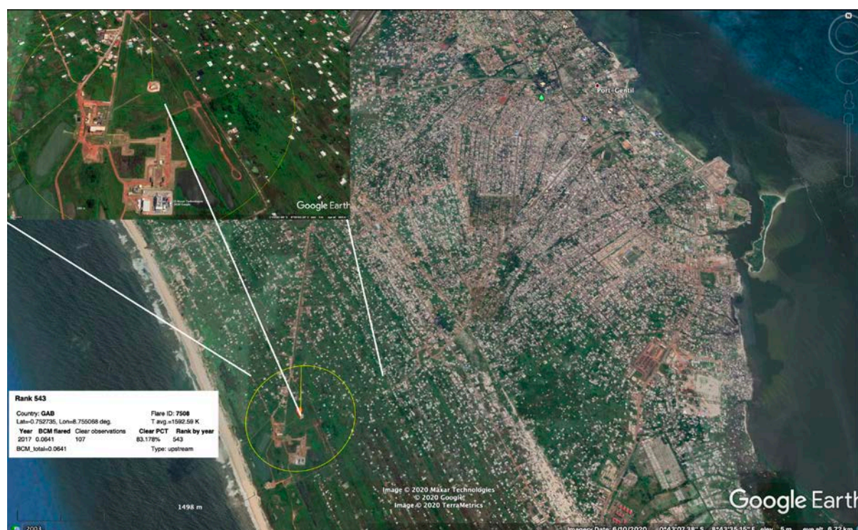
Figure 27b: Contrasting example of a Gabon 6.2 MMscfd gas flare on the outskirts of Port Gentil, globally ranked 543rd in 2017
