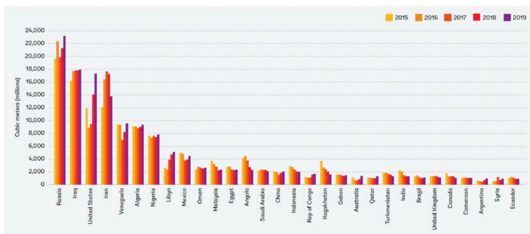
Figure 14: GGFR and 'Zero Routine Flaring by 2030' initiatives need further efforts to reverse the trend of increasing flare volumes
