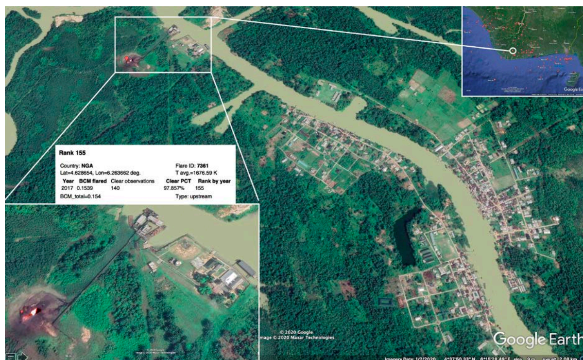
Figure 7: Identification of a flare (ranked 155th) near a village in the Niger Delta in Nigeria
