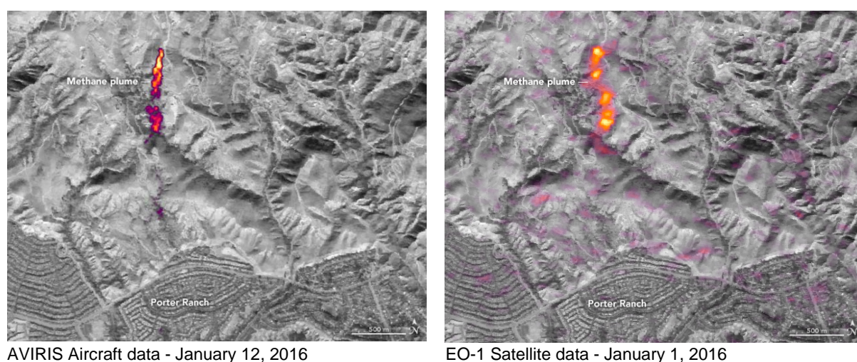
Figure 10: First satellite detection of a methane plume leaking from a single facility in January 2016
