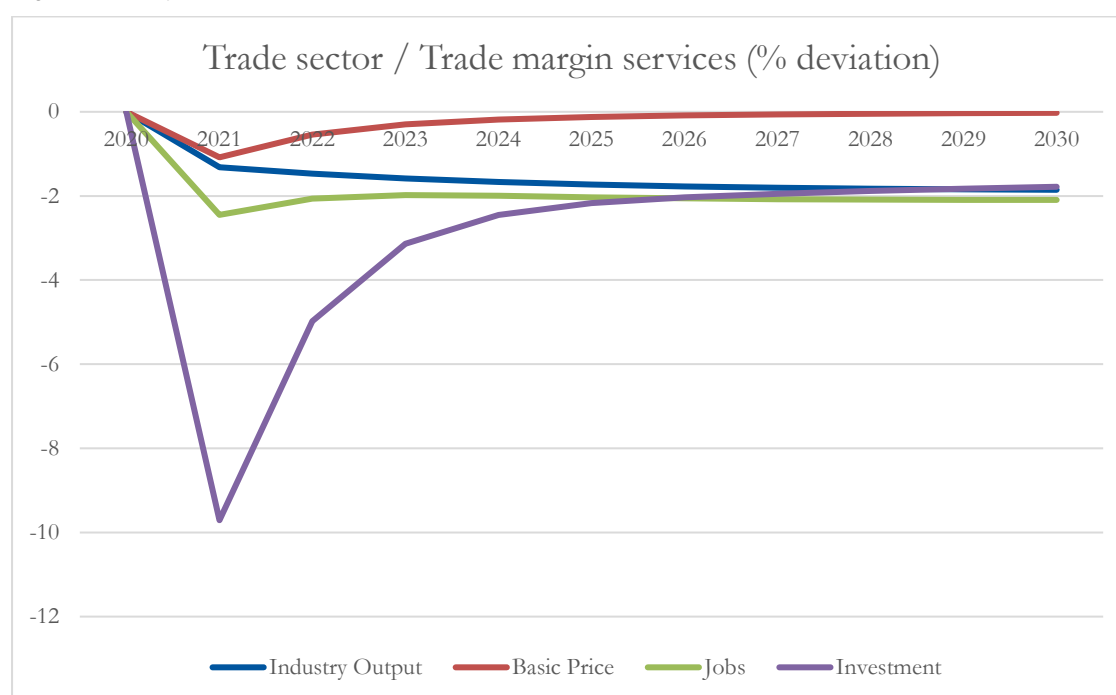
Figure 5: Policy simulation results for S5 combined, 2021–30 (trade sector)
