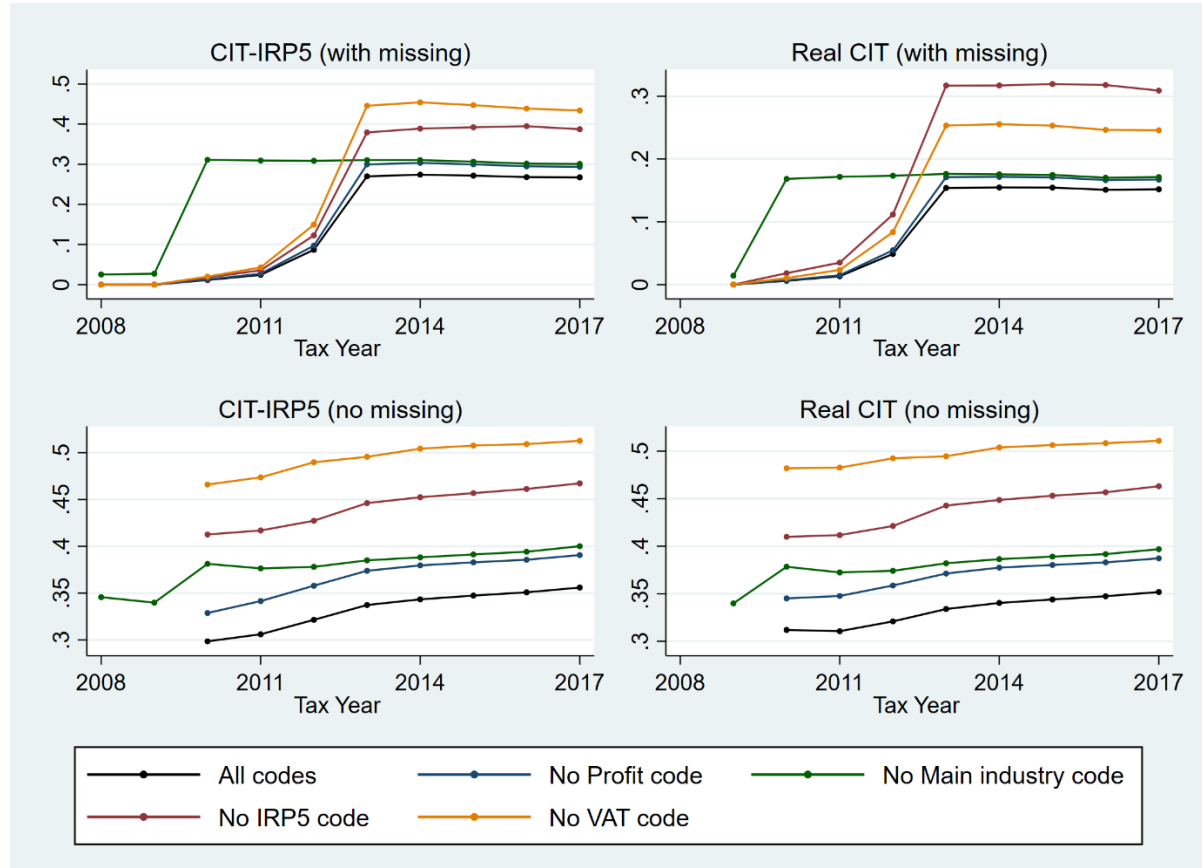
Figure 9: Across-variable agreement for different combinations of industry variables
