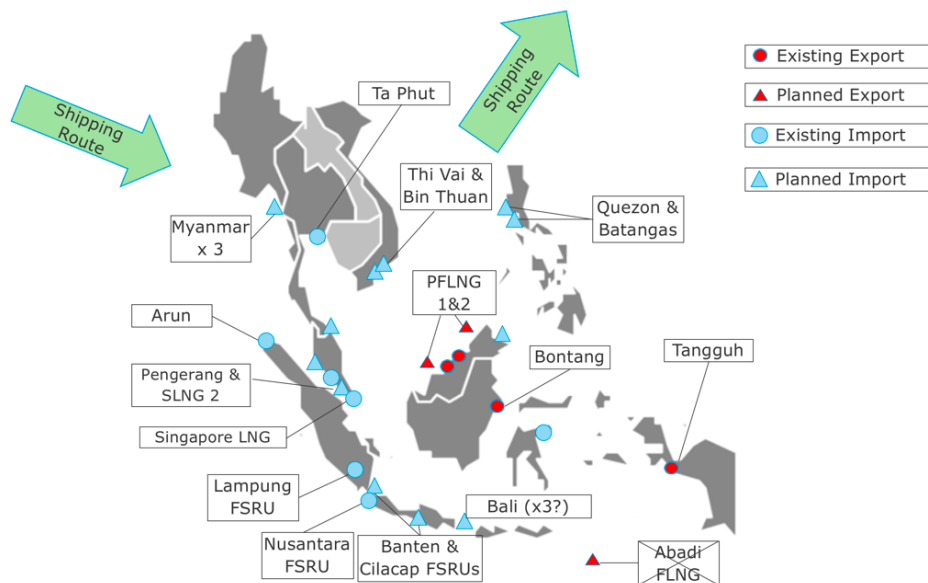
Figure 2: Some large LNG projects in SEA
