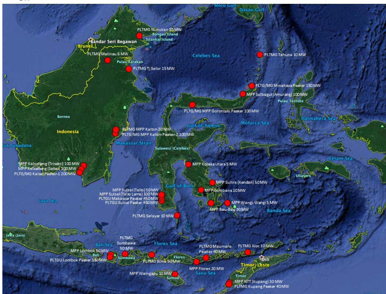
Figure 8: PLN gas fired power projects in Indonesia involving 32 small to large LNG regas facilities for a total 2.8 GW
