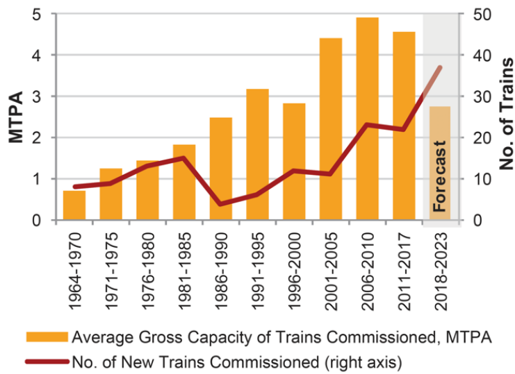
Figure 7: After a period of increasing LNG train sizes to obtain economies of scale from mega LNG developments, the foreseeable trend is now for on average smaller LNG train sizes.
