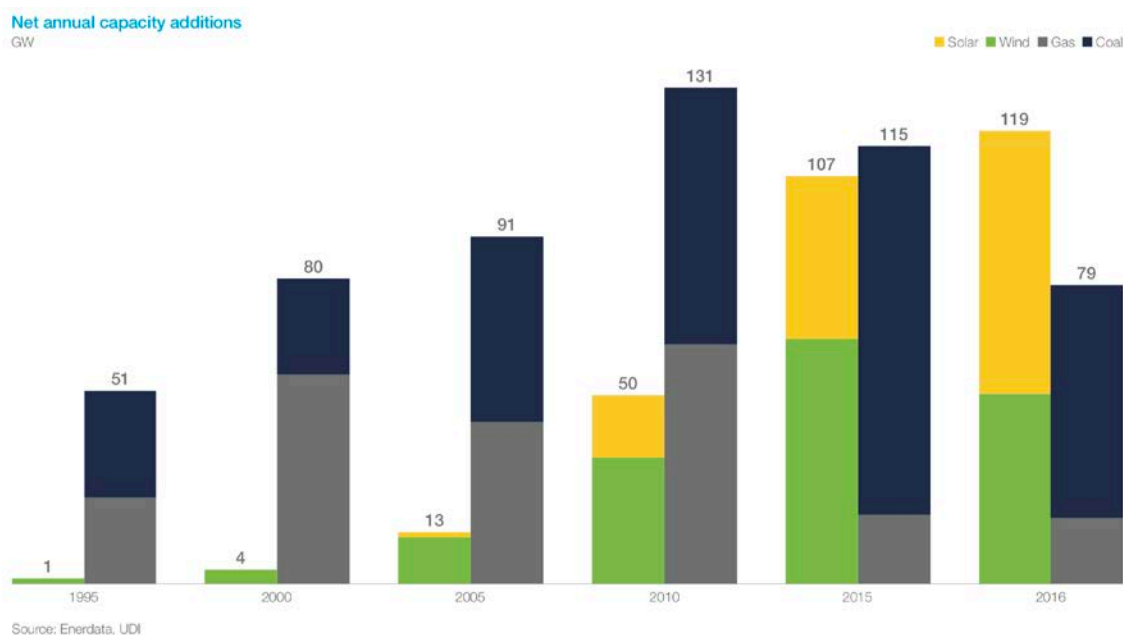
Figure 19: Global net annual power capacity additions in GW
