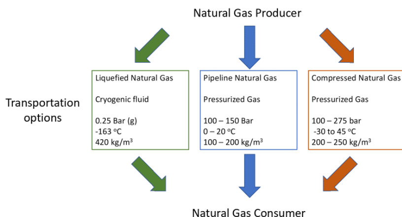
Figure 1: Properties of LNG compared with pipeline NG and CNG
