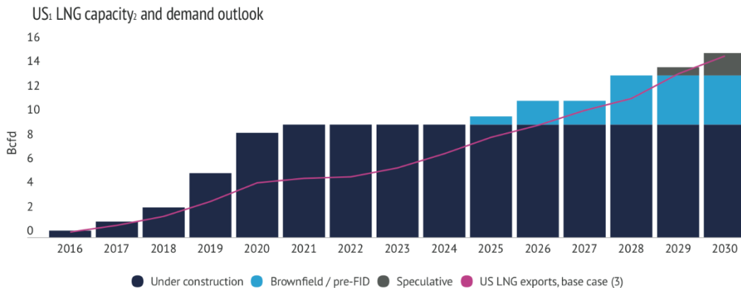
Figure 11: US LNG export capacity and demand outlook (1 Bcfd = 7.6 mtpa of LNG)
