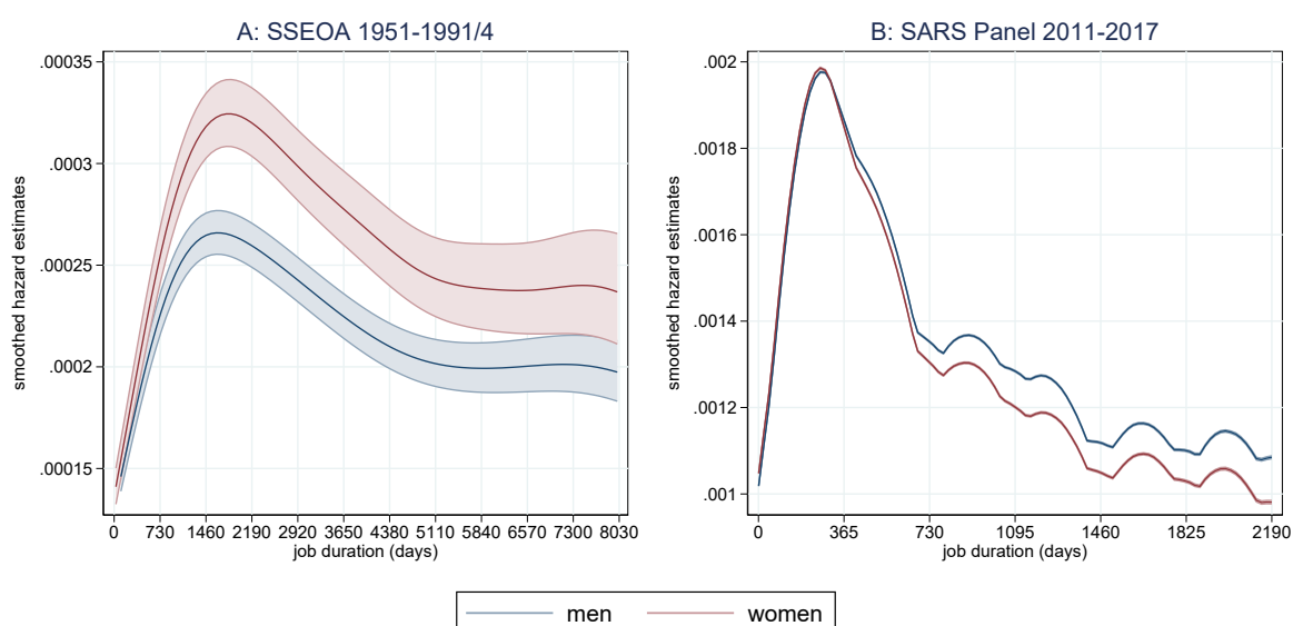
Figure 5: Kaplan–Meier estimates of the job duration hazard in the South African formal sector
