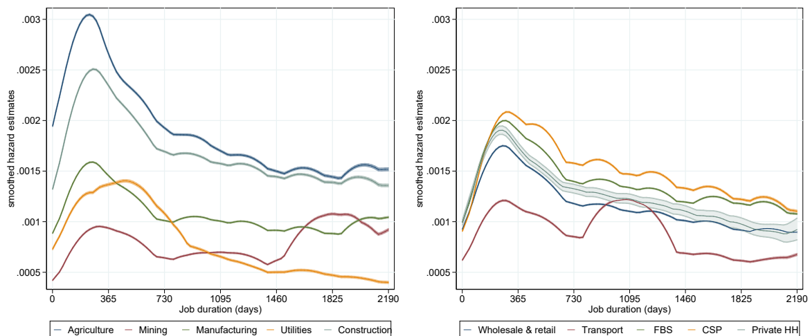
Figure 8: Kaplan–Meier estimates of the job duration hazard in the South African formal sector by industrial sector, 2011–17
