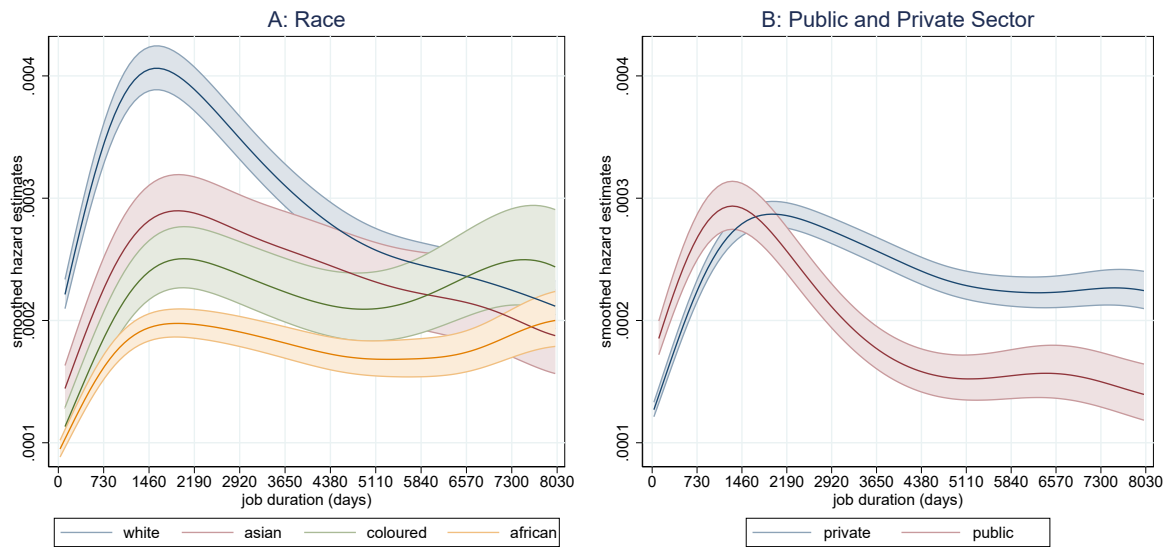
Figure 6: Kaplan–Meier estimates of the job duration hazard in the South African formal sector by race and public sector status, 1951–91/94
