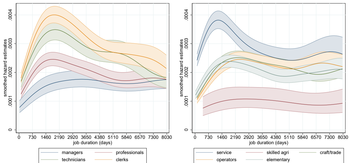
Figure 7: Kaplan–Meier estimates of the job duration hazard in the South African formal sector by occupation, 1951–91/94
