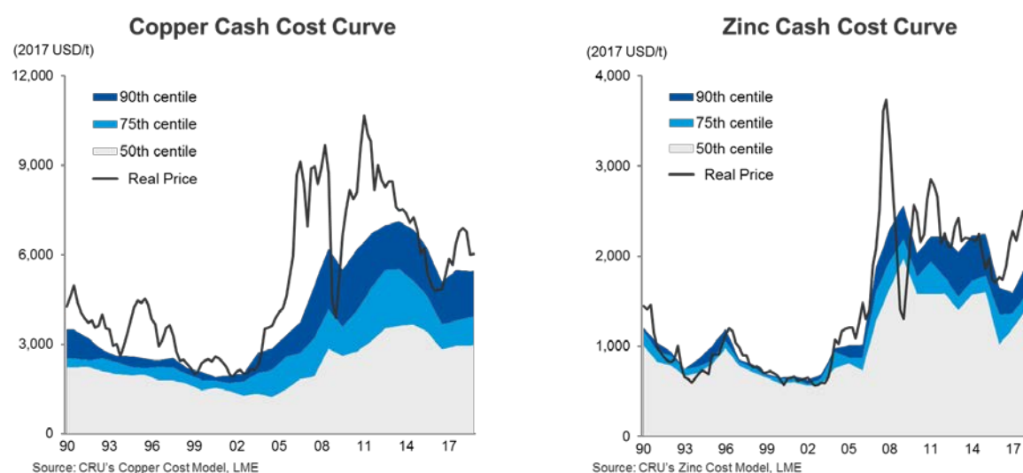
Figure 13: Price and distribution of cash costs in copper and zinc production, US$ per tonne
