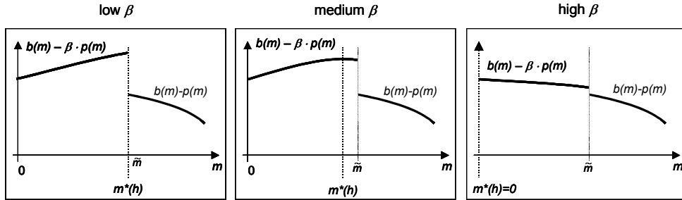
Figure 2: The optimal level of misbehavior in the static problem
