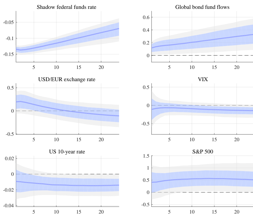
Figure 15: Impulse responses in baseline model with recursive identification
