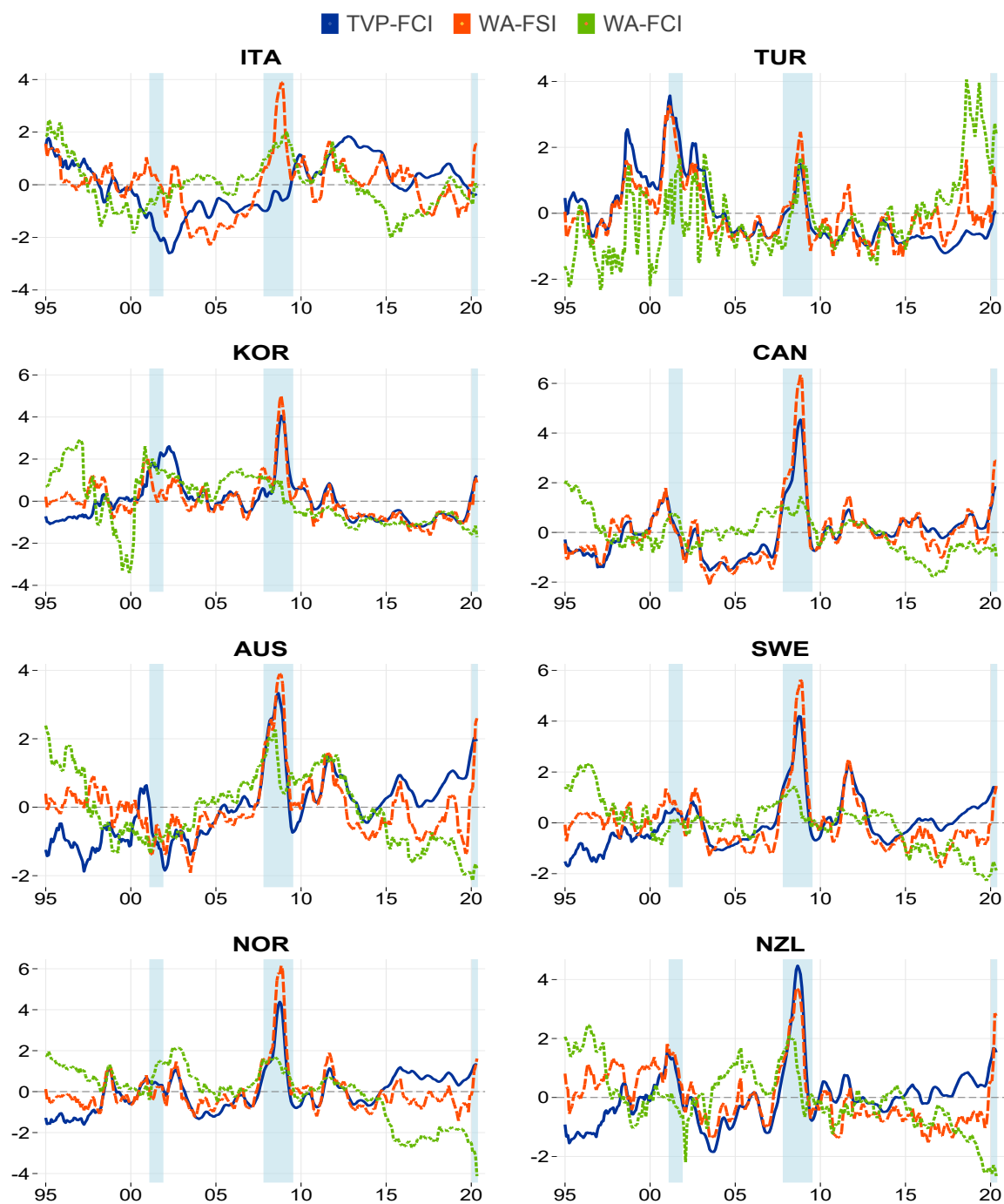
Figure 3b: Comparison of the FCIs, continued
