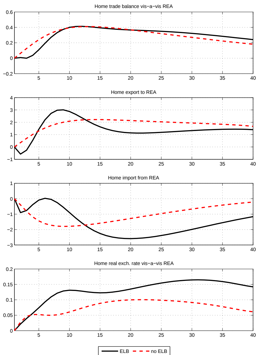
Figure 18: US tariffs, high elasticity, and the ELB: intra-EA trade
