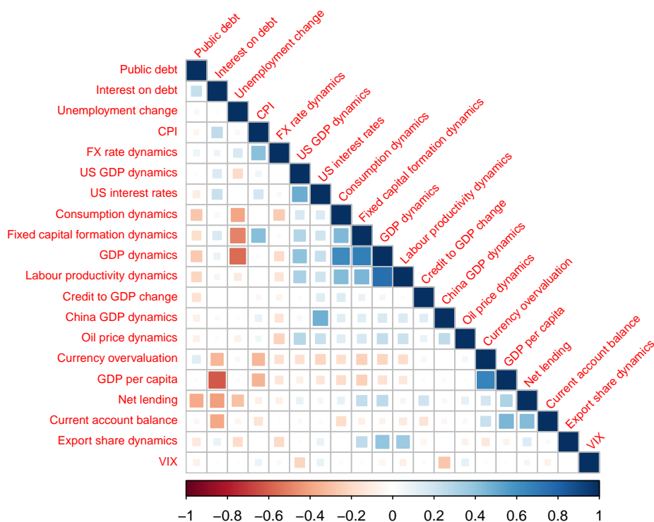
Figure 2: Pairwise Correlations Between the Variables Used in the Analysis
