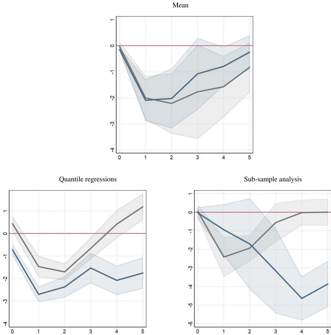
Figure 21: Additional covariates
