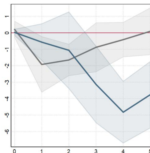
Figure 17: Sub-sample analysis
