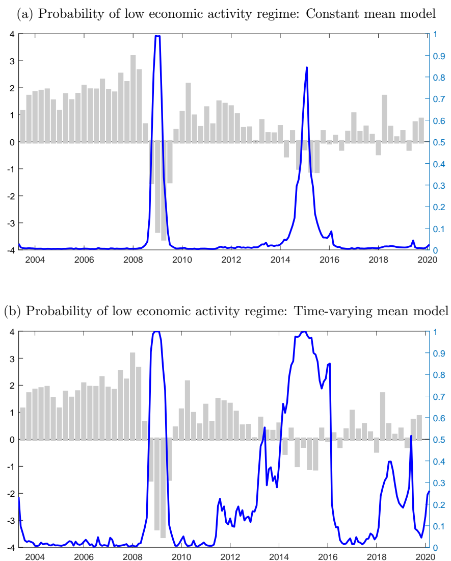
Figure 17: Russia
