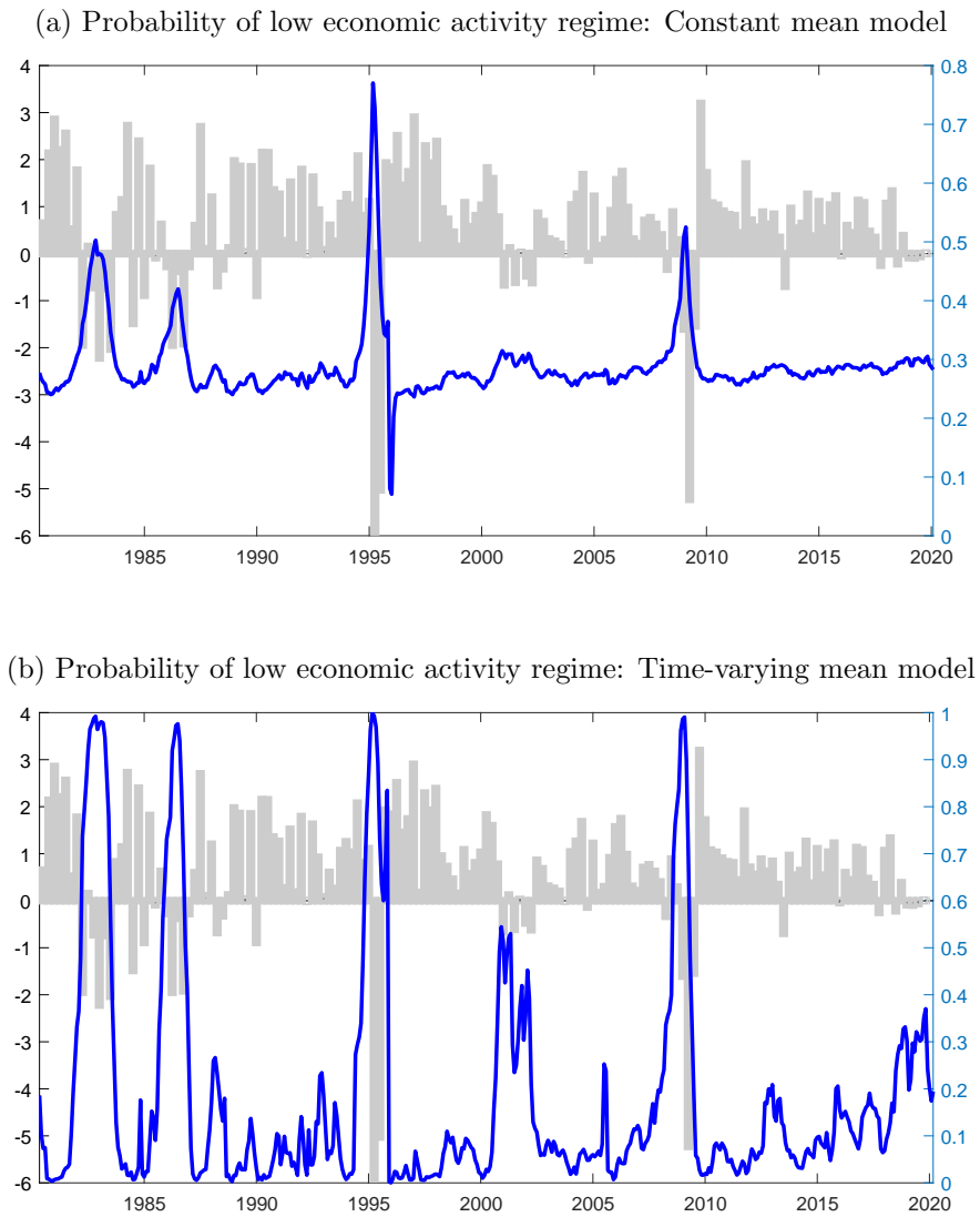
Figure 16: Mexico
