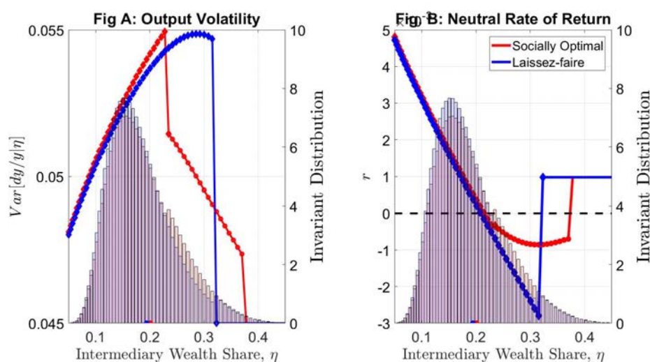
Figure 17: Neutral Rate under Socially Optimal and Laissez-faire Macprudential Policy.
