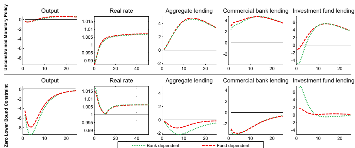
Figure 16: Responses of intermediaries to a demand shock. Note: Horizontal axes show periods in quarters, vertical axes are percentage deviations from steady state.
