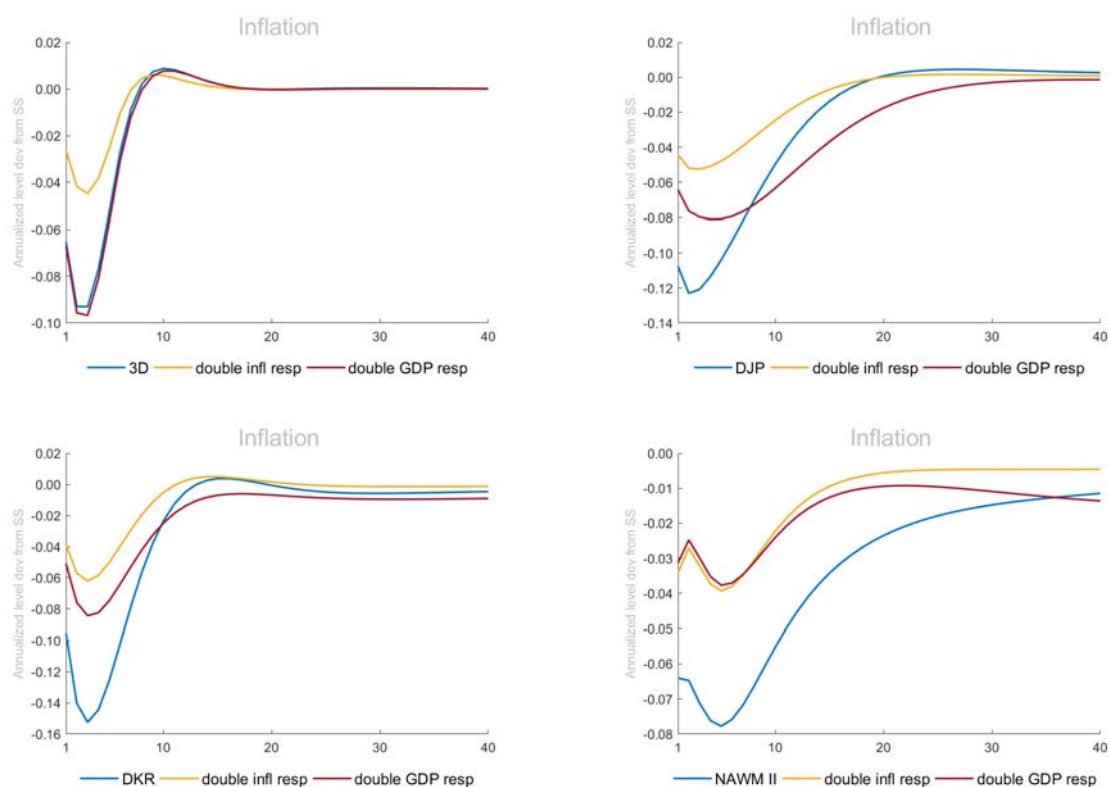
Figure 7: Inflation in the four models.
