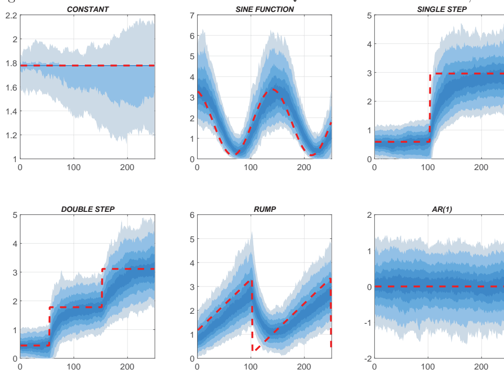
Figure D.5: TIME-VARYING MEASUREMENT EQUATION ERROR VARIANCE, n=250
