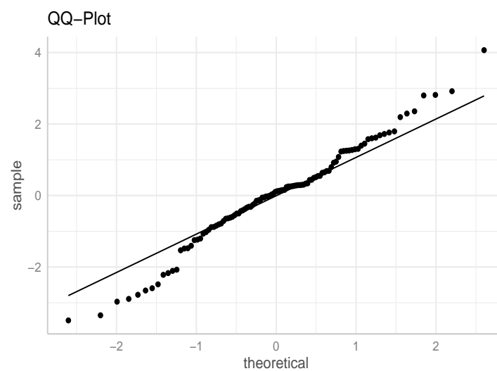
Figure 2: Quantile-Quantile plot
