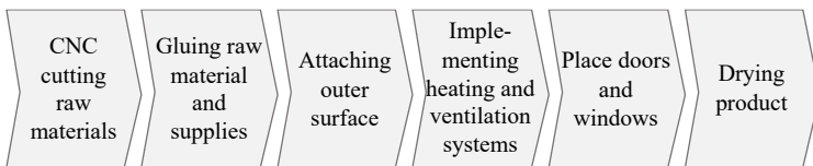
Figure 3: Production steps of a Smart Construction Factory
