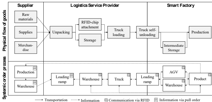
Figure 5: Procurement Logistics concept of a Smart Factory
