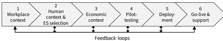
Figure 2: Procedural model for exoskeleton implementation in intralogistics
