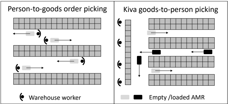
Figure 2: Classic order picking vs Kiva picking
