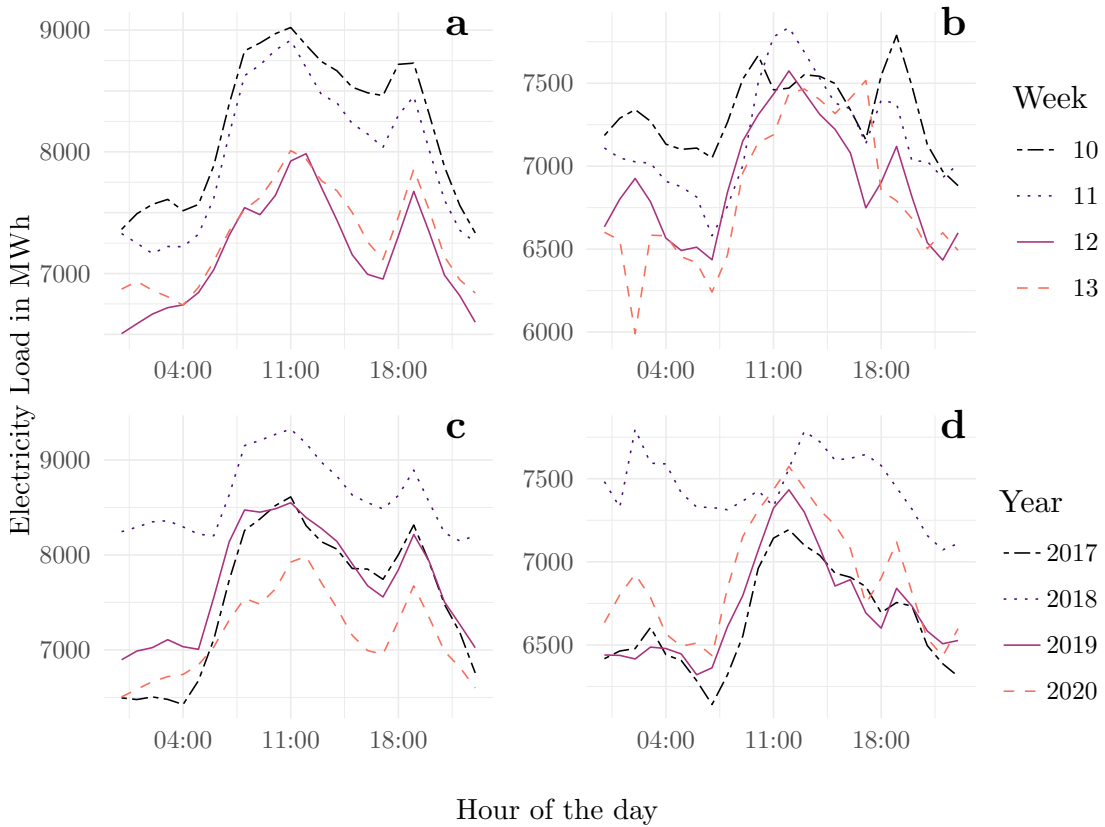
Figure 1: Average Daily Load Profiles in Switzerland
