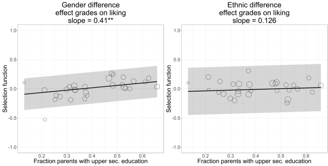
Figure 3: Varying group differences in the effect of grades on liking across schools with different fractions of parents with an upper secondary education.
