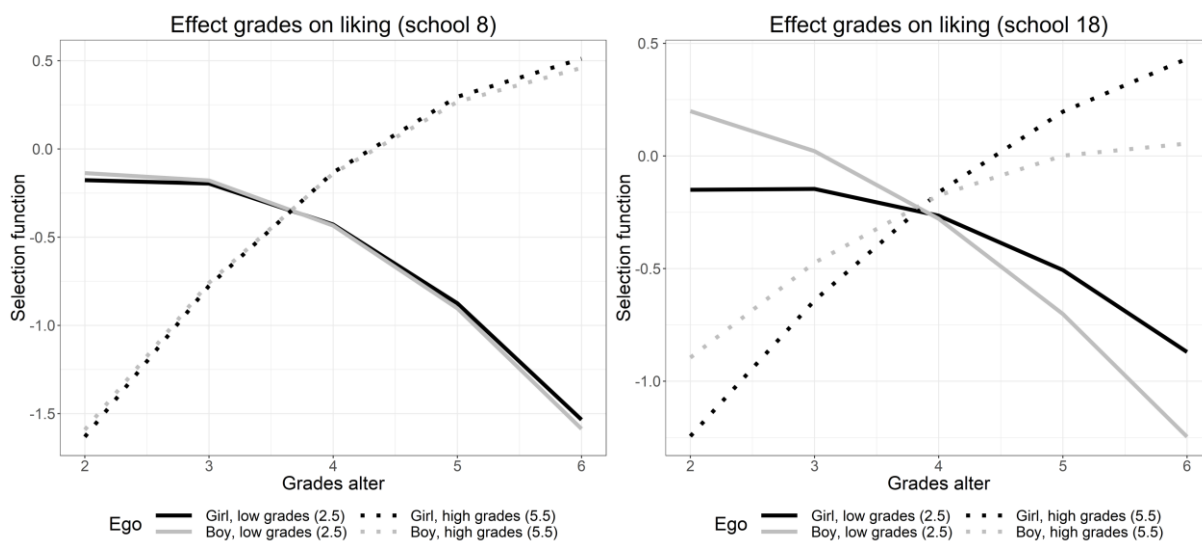
Figure 2. Selection effects related to students' grades in two example schools.
