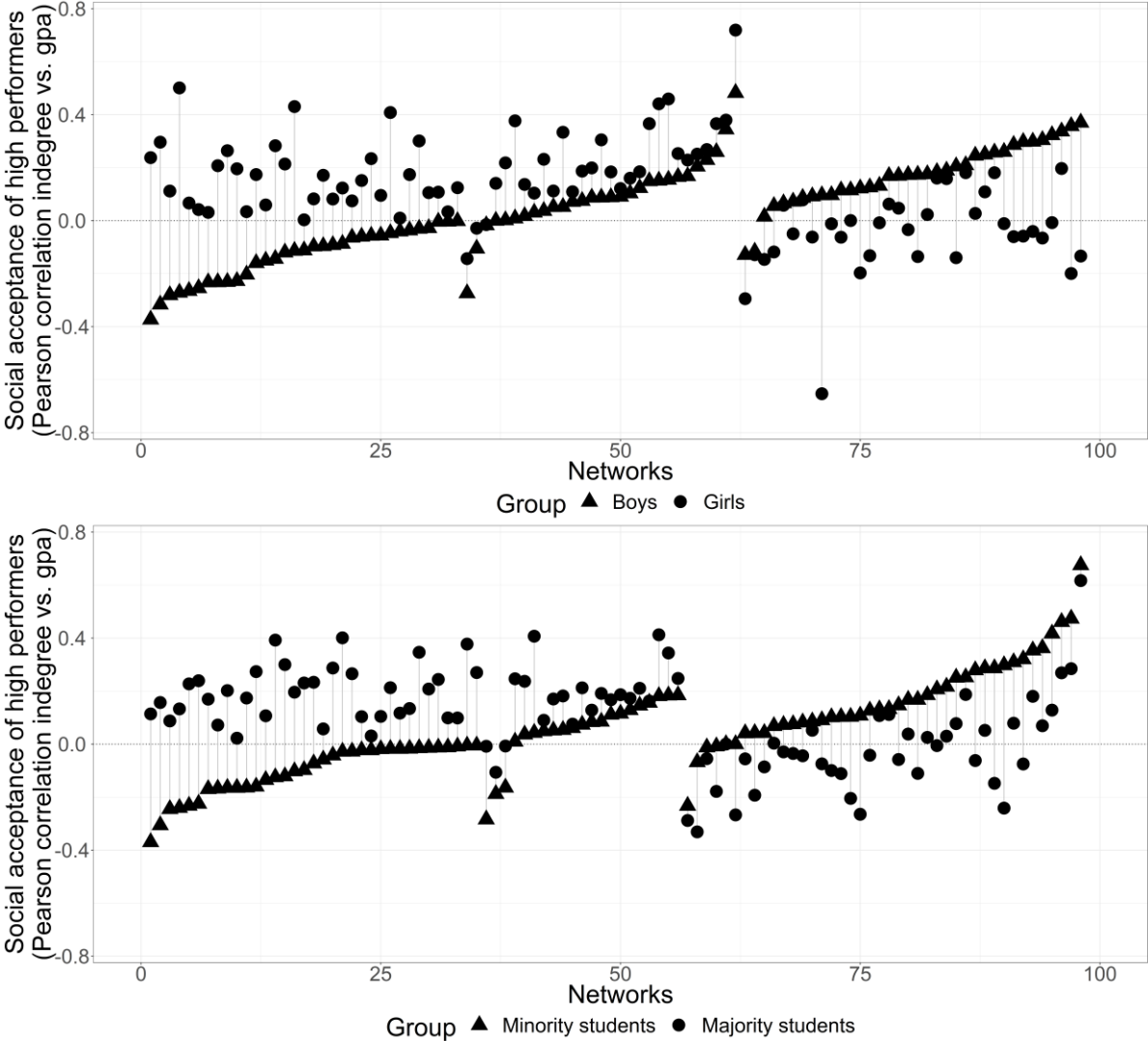
Figure 1: Gender-specific (upper panel) and ethnicity-specific (lower panel) associations between students' social acceptance (liking indegrees) and their school performance (grade point averages) across all school grades and observed time points in the analytic sample.
