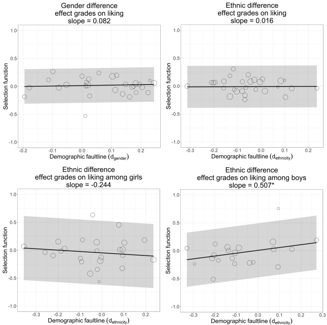
Figure 4: Varying group differences in the effect of grades on liking across schools with different demographic faultlines.
