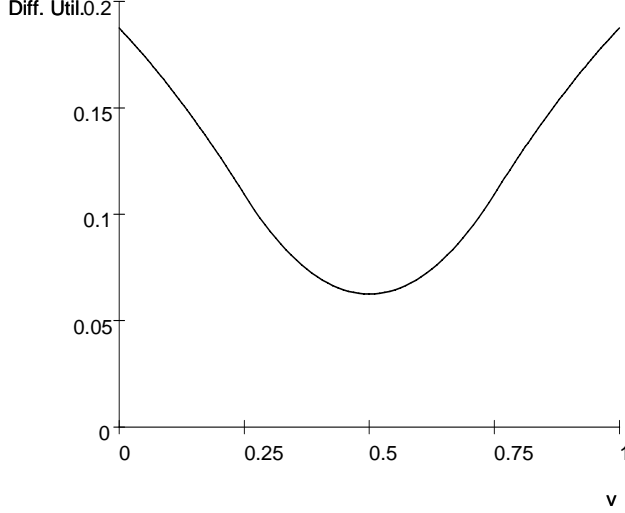
Figure 2: U^C(v) - U^P(v) for uniform distribution.
