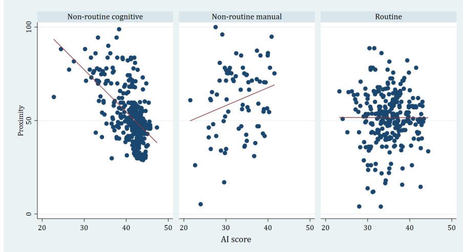
Figure 2: Scatterplot of AI impact score and physical proximity by routine-intensity. Source: Author's calculations.
