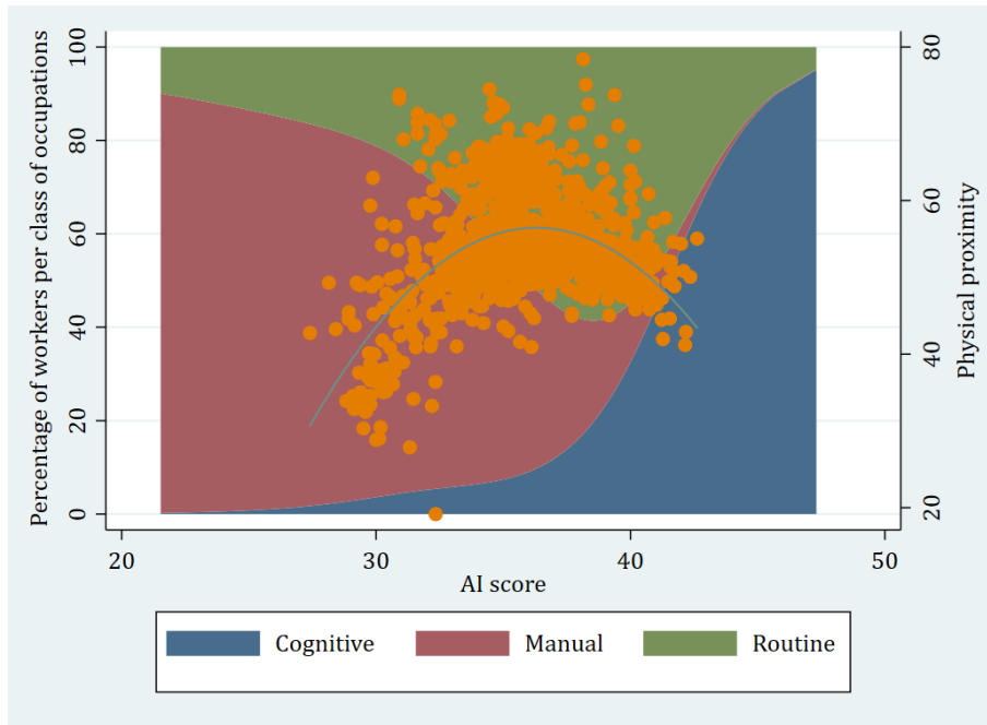
Figure 3: Share of workers across classes of occupations together with (mean) AI impact score and (mean) physical proximity for 1222 industries. Source: Author's calculations.
