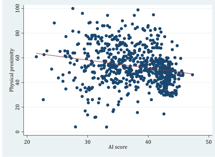
Figure 1: Scatterplot of AI impact score and physical proximity for 697 occupations. Source: Author's calculations.
