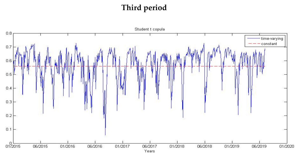
Figure 3. Time varying Student t copula for Kansas-MATIF price pair.
