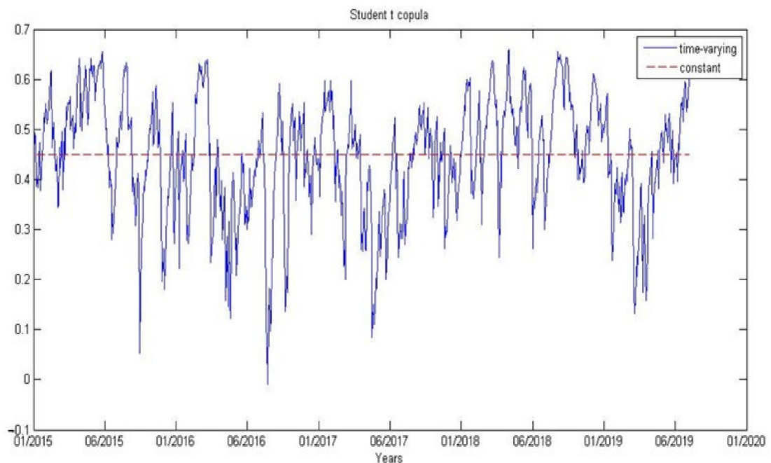
Figure 4. Time varying Student t copula for Minneapolis-MATIF price pair.
