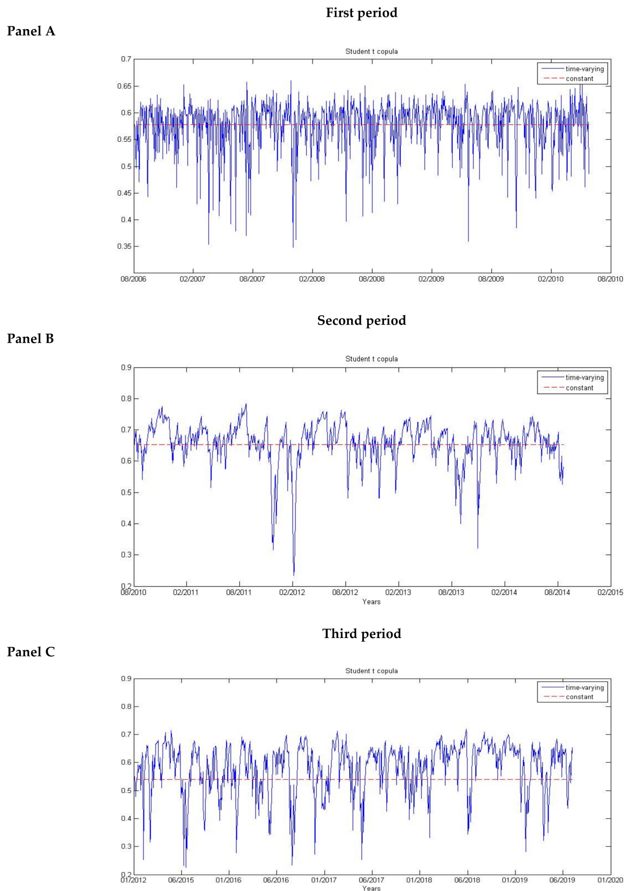
Figure 2. Time varying Student t copula for CBOT-MATIF price pair.
