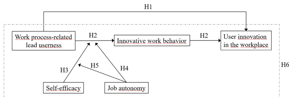
Fig. 1. Hypothesized relationships.
