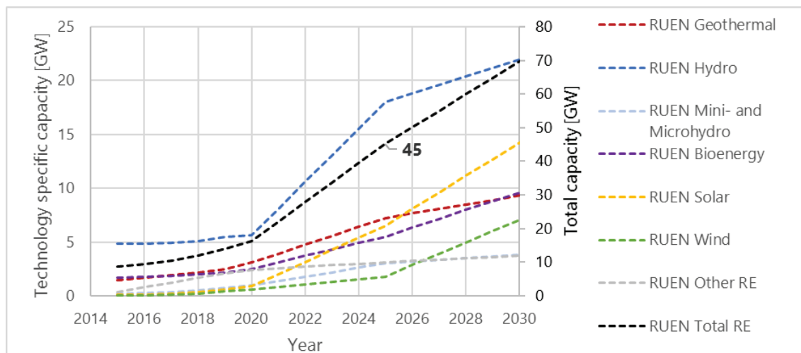
Figure 3: Renewable energy capacity plan as given in RUPTL
