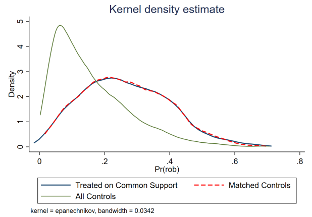
(b) NNmatching-ThreeNeighbours
