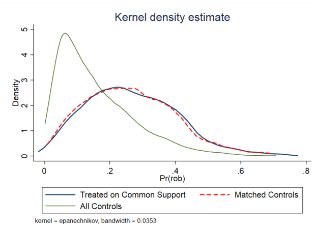
(c) KernelMatching
