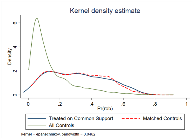
(a) NNmatching-VariablesInLevels
