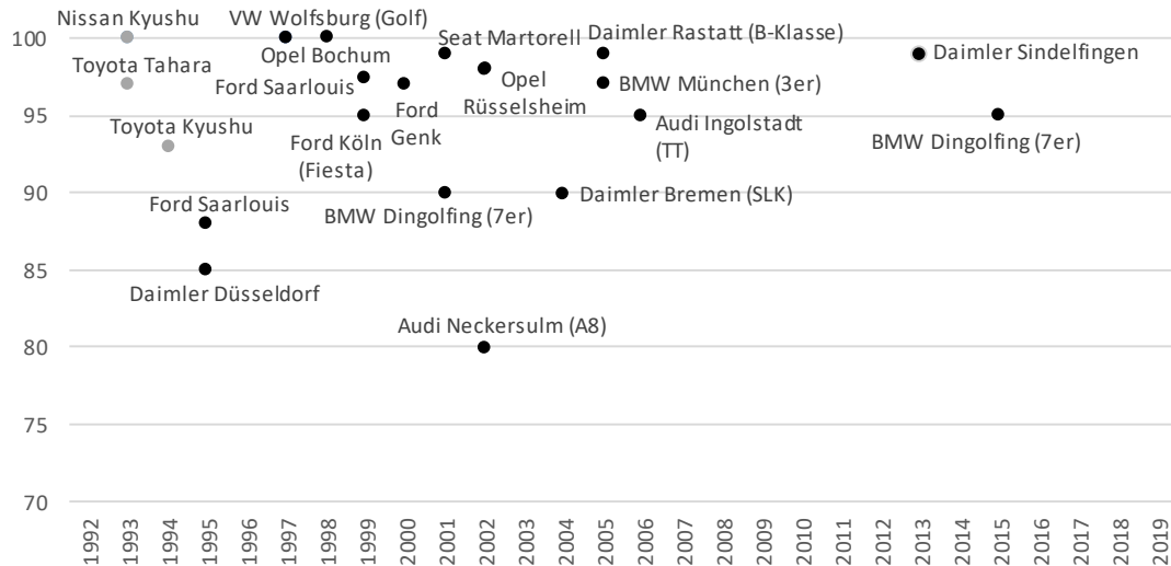
Figure 1: Body shop automation levels of selected automobile plants
