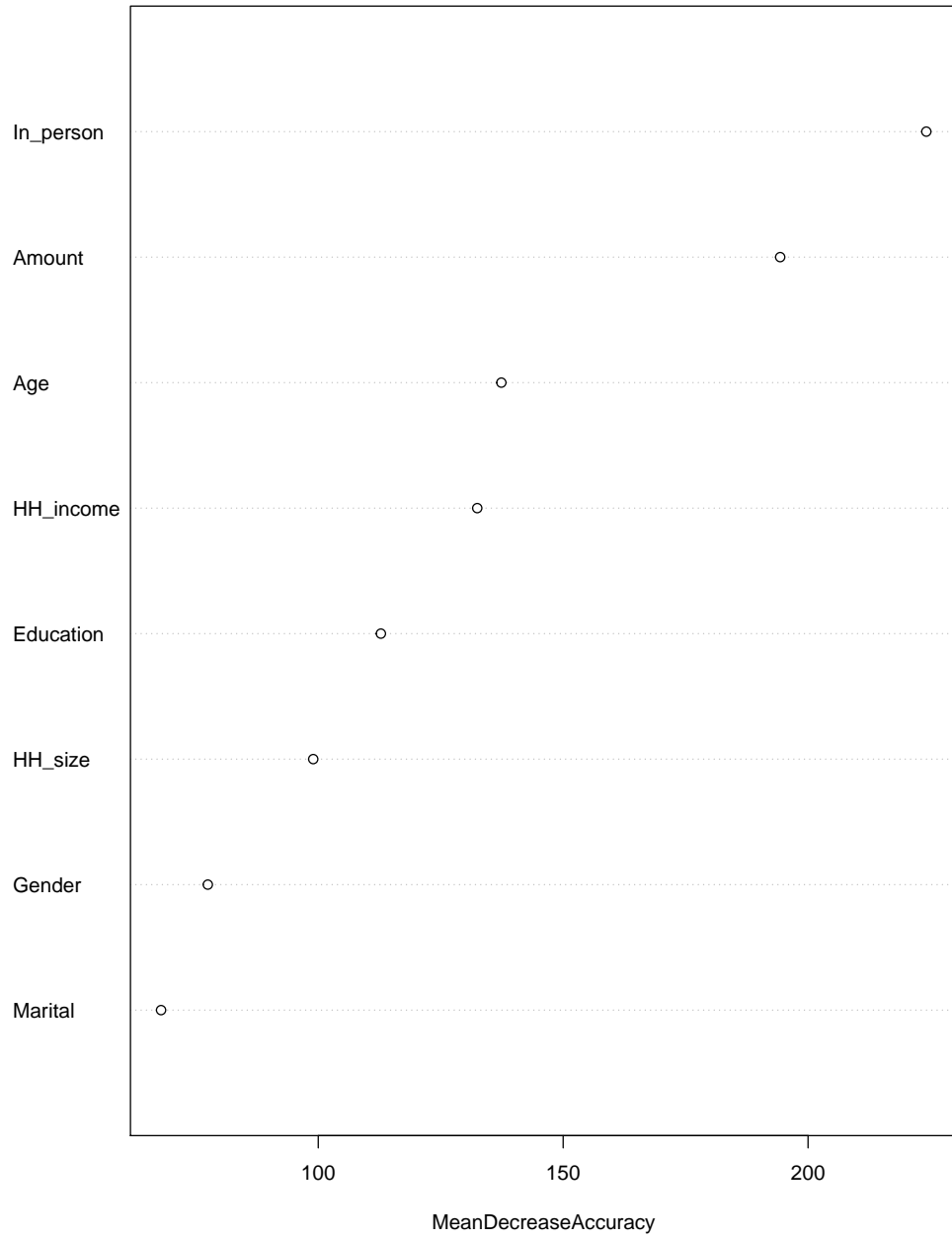
Figure 2: Variable importance plot (VIP) generated by random forest.
