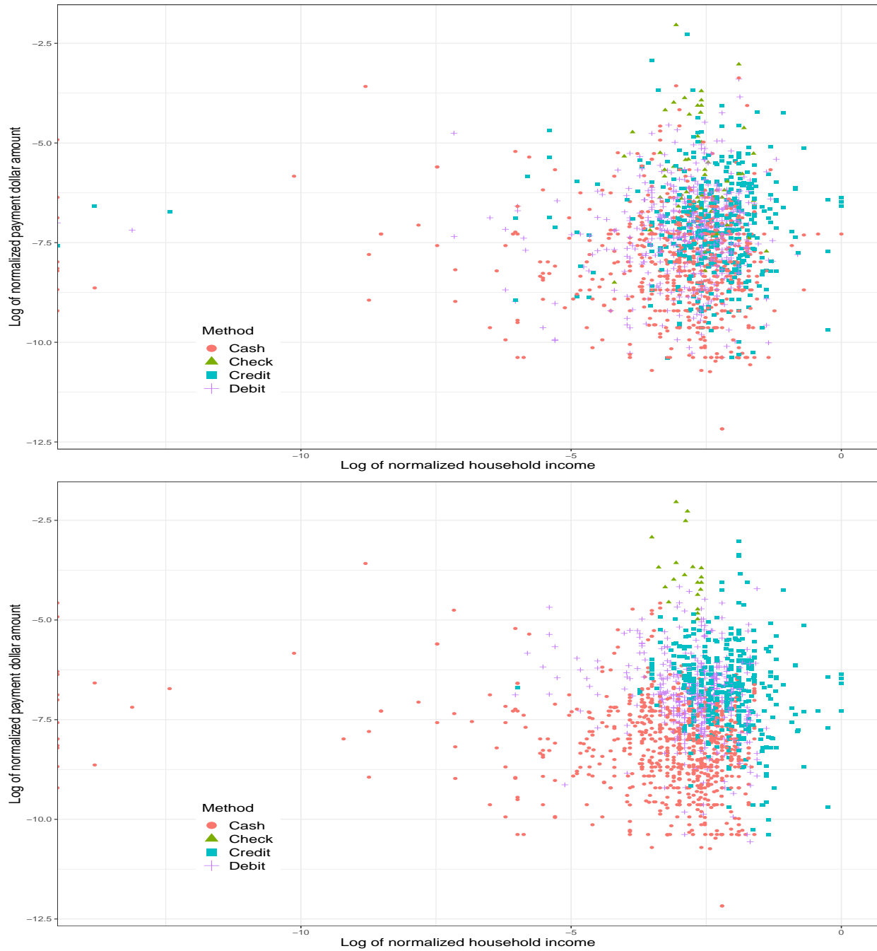
Figure 3: k NN classifications of in-person payment methods in the space of two features: Amount and household income.
