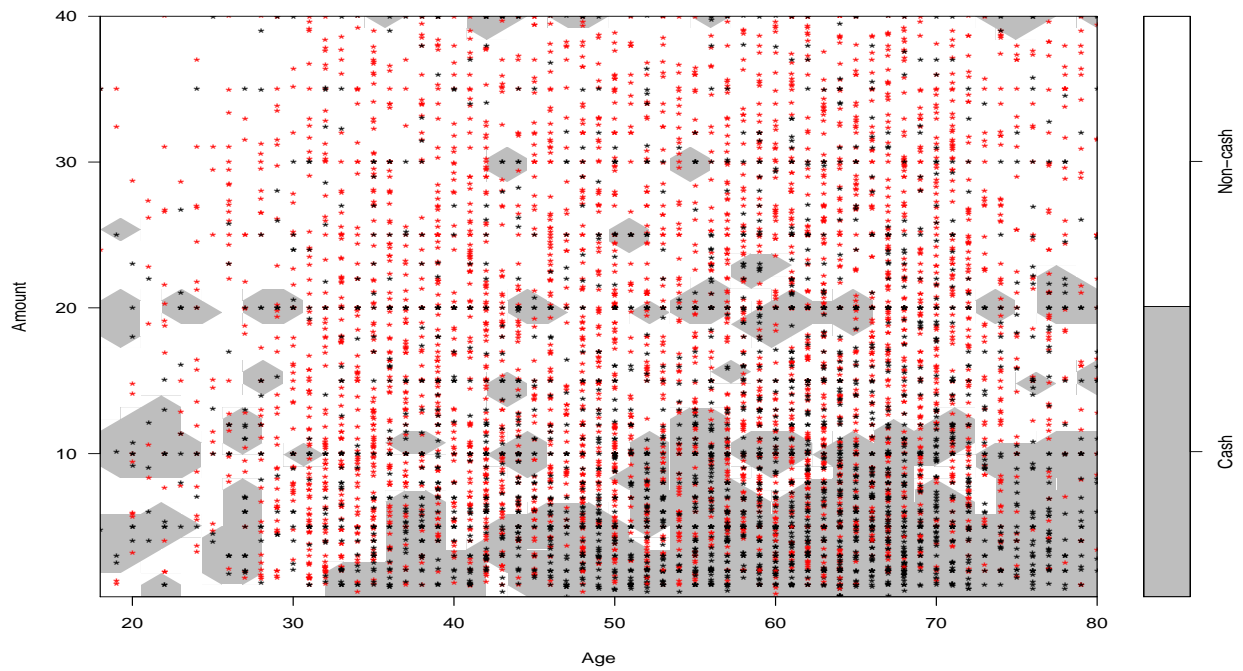
Figure 4: SVM payment method classifications in the space of two features: Amount and age.
