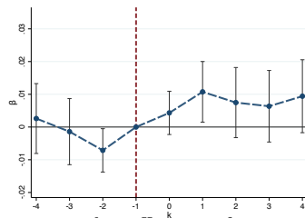
(e) \beta_{T,P}
