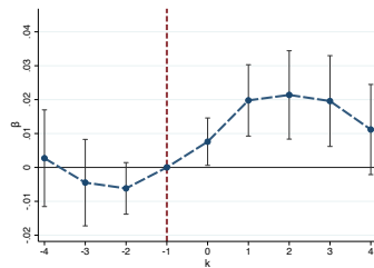
(c) \beta_{T,P}
