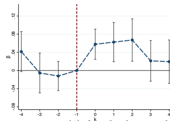
(f) \beta_{rev,P}
