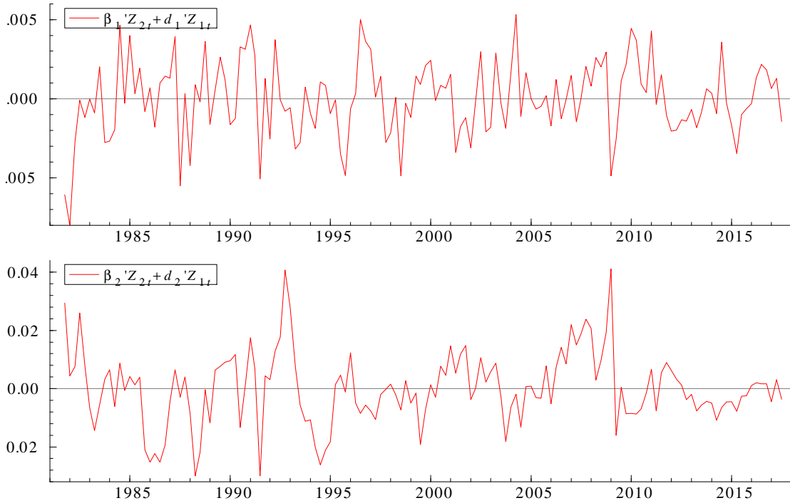
Figure 7: Multi-cointegrating relations
