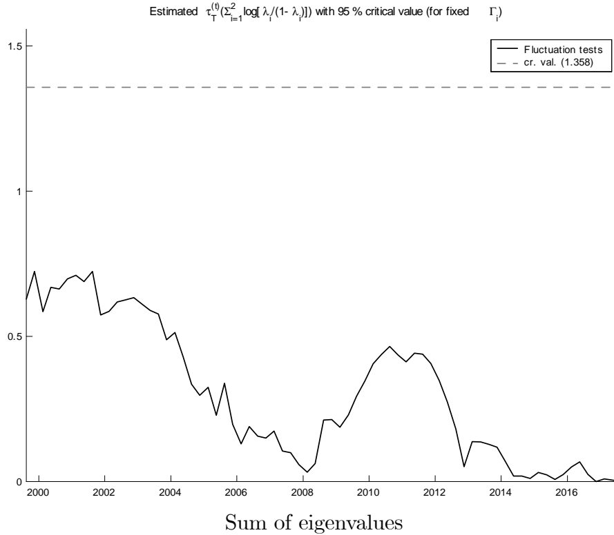
Figure 6: Fluctuation test and 95 per cent critical value
