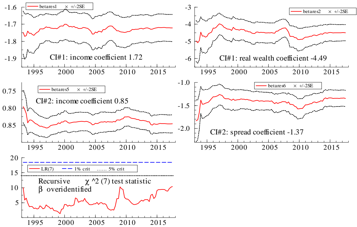
Figure 4: Recursive estimates
