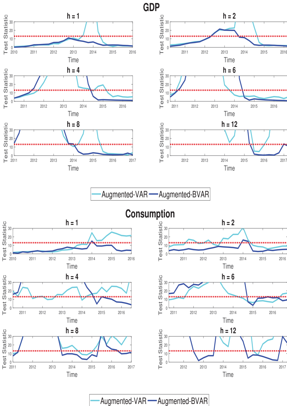
FIGURE 16. Rossi and Sekhposyan (2016) Rationality Test.
