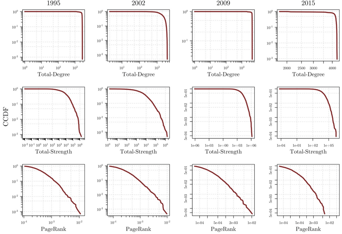
Figure 4 Distributions of Degree, Strength and PageRank Centralities, Selected Years
