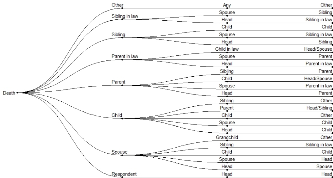
Figure B.1: Classification algorithm
