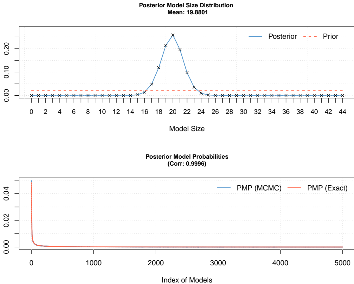
Figure A3: Alternative BMA priors - Model size and convergence
