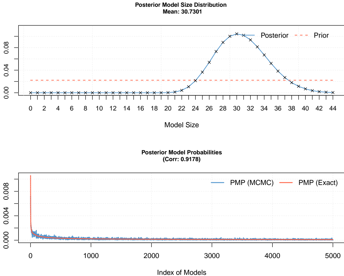
Figure A5: Alternative BMA priors - Model size and convergence
