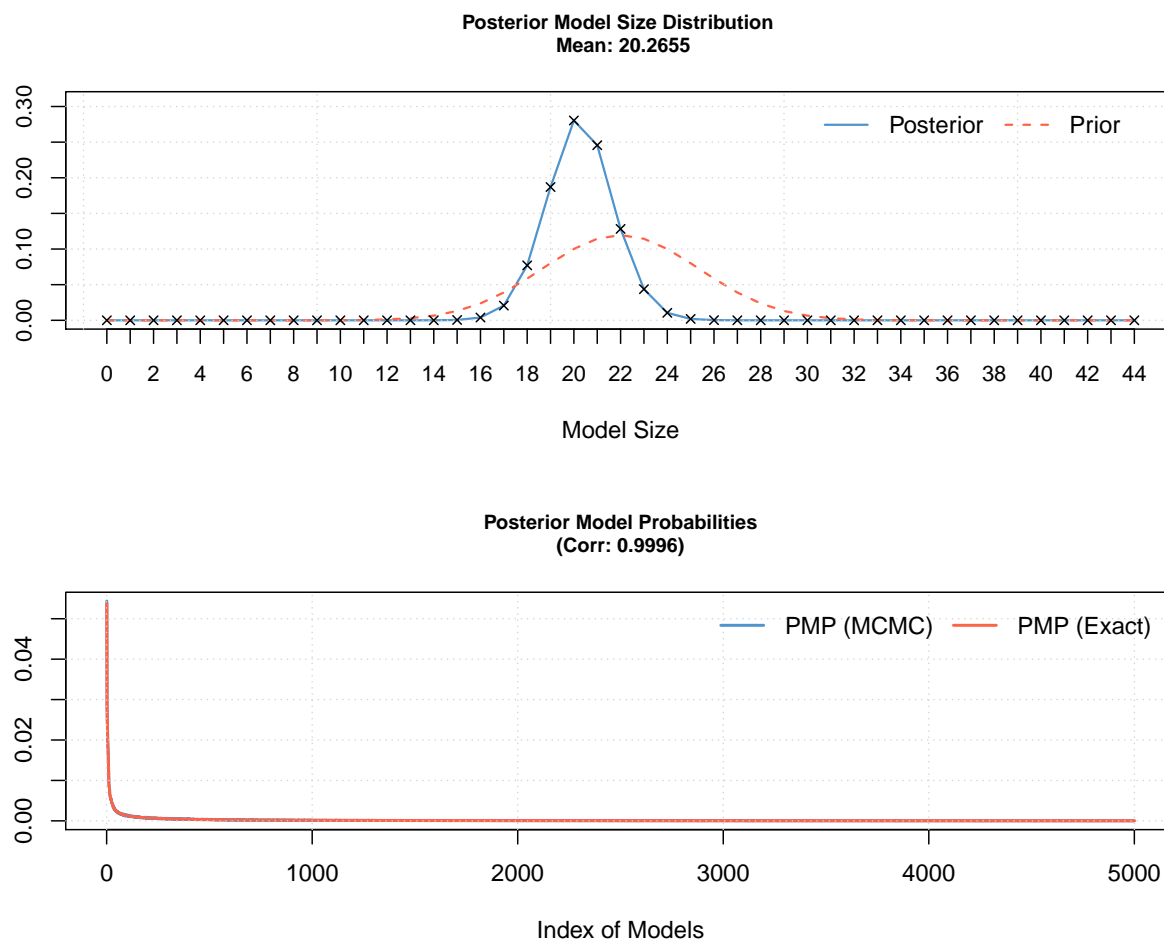
Figure A1: Baseline BMA - Model size and convergence
