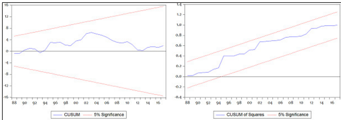
Figure 2: CUSUM &amp; CUSUMSQUARE for Stability within 5% Critical Level
