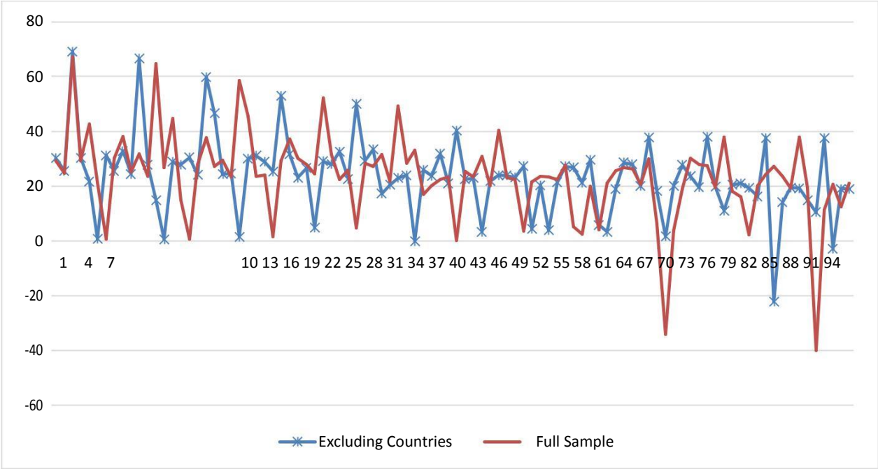
Figure 2: Comparing Residuals of the Initial Regression in Table 5 and Regression from Sensitivity Check
