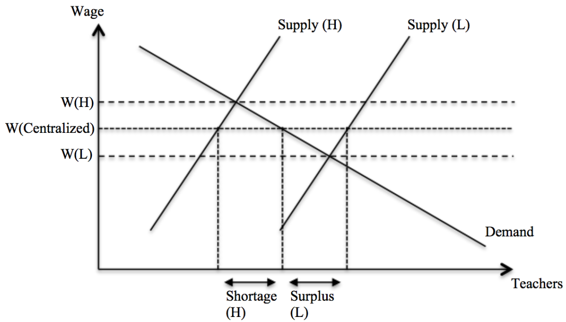
Figure 2: Centralized wage-setting
