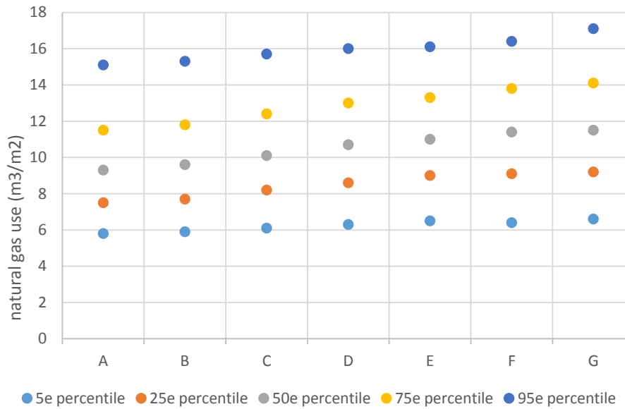
Figure 19. Distribution of temperature-corrected natural gas consumption figures in intermediate houses, use surface area 100 to 150 m 2 , built in 1975 to 1992, 2016 (m 3 /m 2 ) per label
