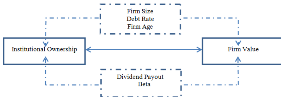
Figure 1. Theoretical Framework
