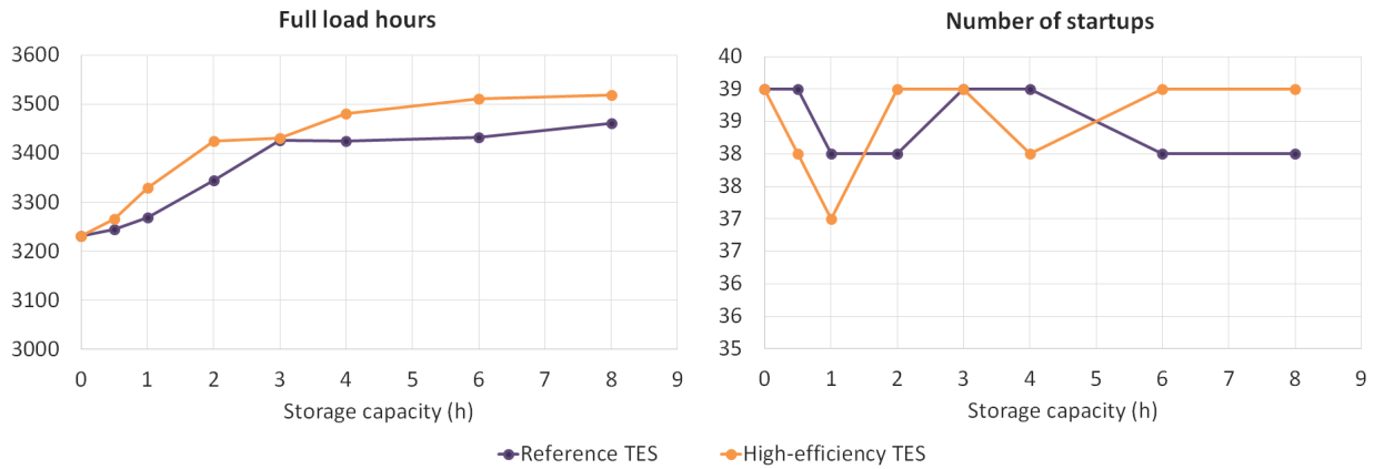
Figure 3: Impact of TES on overall plant dispatch characteristics
