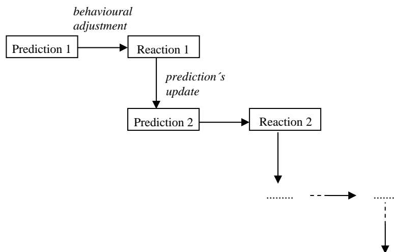
Fig. 2: The Morgenstern Process (from Lehmann-Waffenschmidt, 1990, p. 149)
