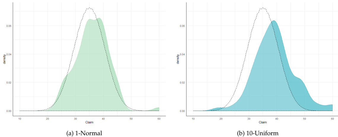
Note: Kernel density of observed claims in both conditions: 1-Normal (Panel 4a) and 10-Uniform (Panel 4b). Dotted lines represent the expected frequency.
