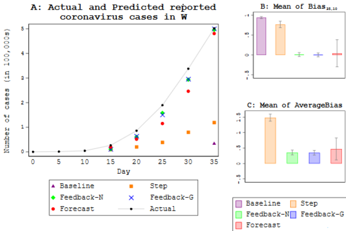
Figure 1: Prediction Bias
