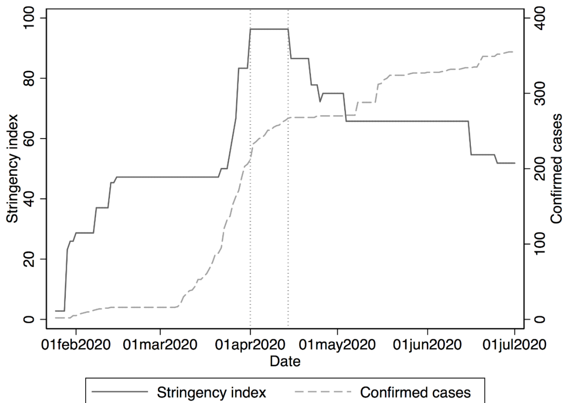
Figure A1: Stringency index and confirmed cases
