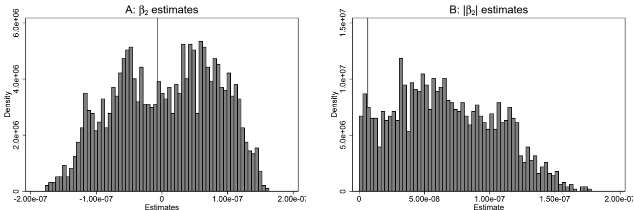
Figure 5: Distribution of \hat{\beta}_2 estimates
