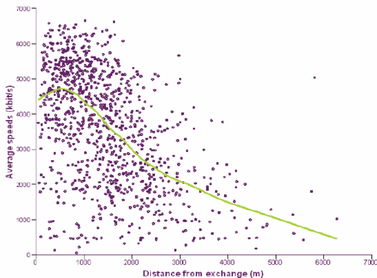
Figure 7.6 Distance from exchange and average download speeds achieved by panellists on packages of 'up to' 8Mbit/s
