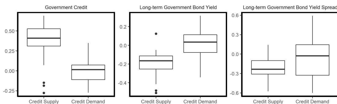
Figure 4: Loadings of public sector credit factors.
