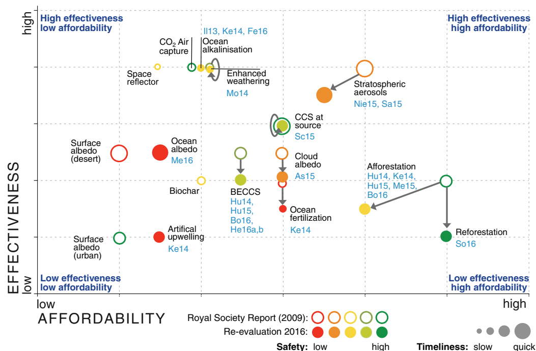
Figure 1. Update of the “blob” diagram of the Royal Society [2009] report that assessed individual CE ideas with respect to the dimension’s effectiveness (vertical), affordability (horizontal), timeliness (blob size), and safety (color). Arrows indicate the direction of change in the assessment by new studies since the Royal Society report. Abbreviations in blue refer to the first letters of the first author’s name and year of the respective publication of the Priority Program [Ilyina et al. , 2013; Humpenöder et al. , 2014, 2015; Moosdorf et al. , 2014; Aswathy et al. , 2015; Mengis et al. , 2015, 2016; Saxler et al. , 2015; Bonsch et al. , 2016; Sonntag et al. , 2016 in addition to references cited elsewhere in the paper], all provided in the reference list of this article.
