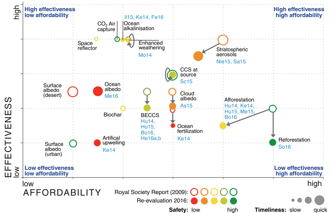
Figure 1. Update of the “blob” diagram of the Royal Society [2009] report that assessed individual CE ideas with respect to the dimension’s effectiveness (vertical), affordability (horizontal), timeliness (blob size), and safety (color). Arrows indicate the direction of change in the assessment by new studies since the Royal Society report. Abbreviations in blue refer to the first letters of the first author’s name and year of the respective publication of the Priority Program [Ilyina et al. , 2013; Humpenöder et al. , 2014, 2015; Moosdorf et al. , 2014; Aswathy et al. , 2015; Mengis et al. , 2015, 2016; Saxler et al. , 2015; Bonsch et al. , 2016; Sonntag et al. , 2016 in addition to references cited elsewhere in the paper], all provided in the reference list of this article.
